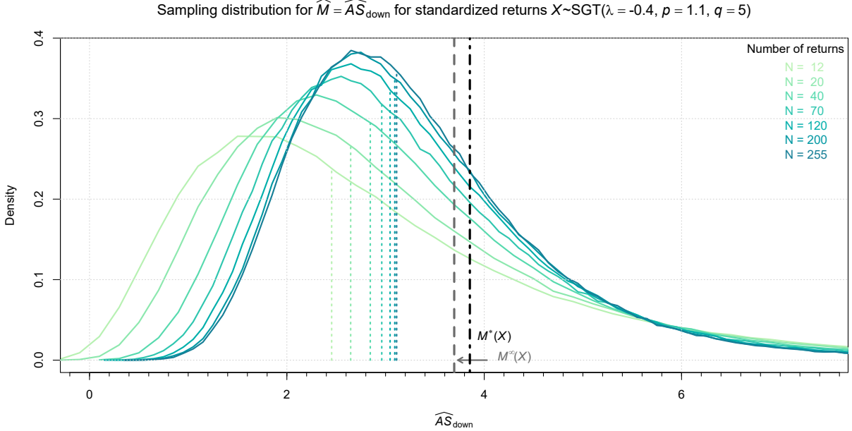
Figure 3: Sampling distributions for the asigma method, i.e. using the estimator \widehat{M} = \widehat{A}\widehat{S}_{\text{down}} for different sample sizes N of overlapping returns X drawn from an SGT distribution (cf. Annex B). The (slow) convergence to the normal distribution is visible for the largest N . The black dot-dashed black vertical line is the true value for the ES, M^* , the short-dashed grey vertical line is the large N limit M^\infty . The estimator exhibits a bias for all N due to the choice of C_{\text{ES}}^{\text{asigma}} = 3 . The vertical dotted lines indicate the median values \text{med}(\widehat{M}) of the sampling distributions for different N , converging to M^\infty .
